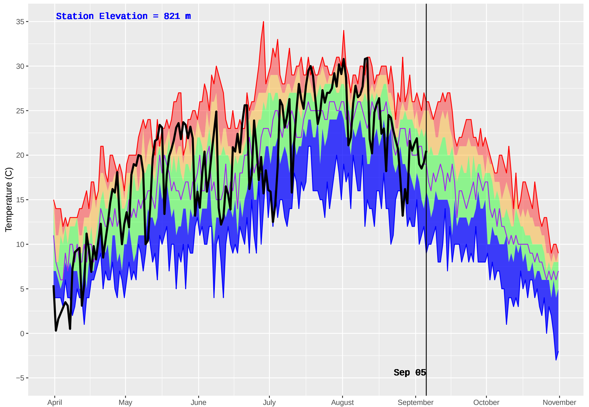
AKOKLI CREEK (838) : Historical (2003–2016) and Current (2018) Daily Temperature
