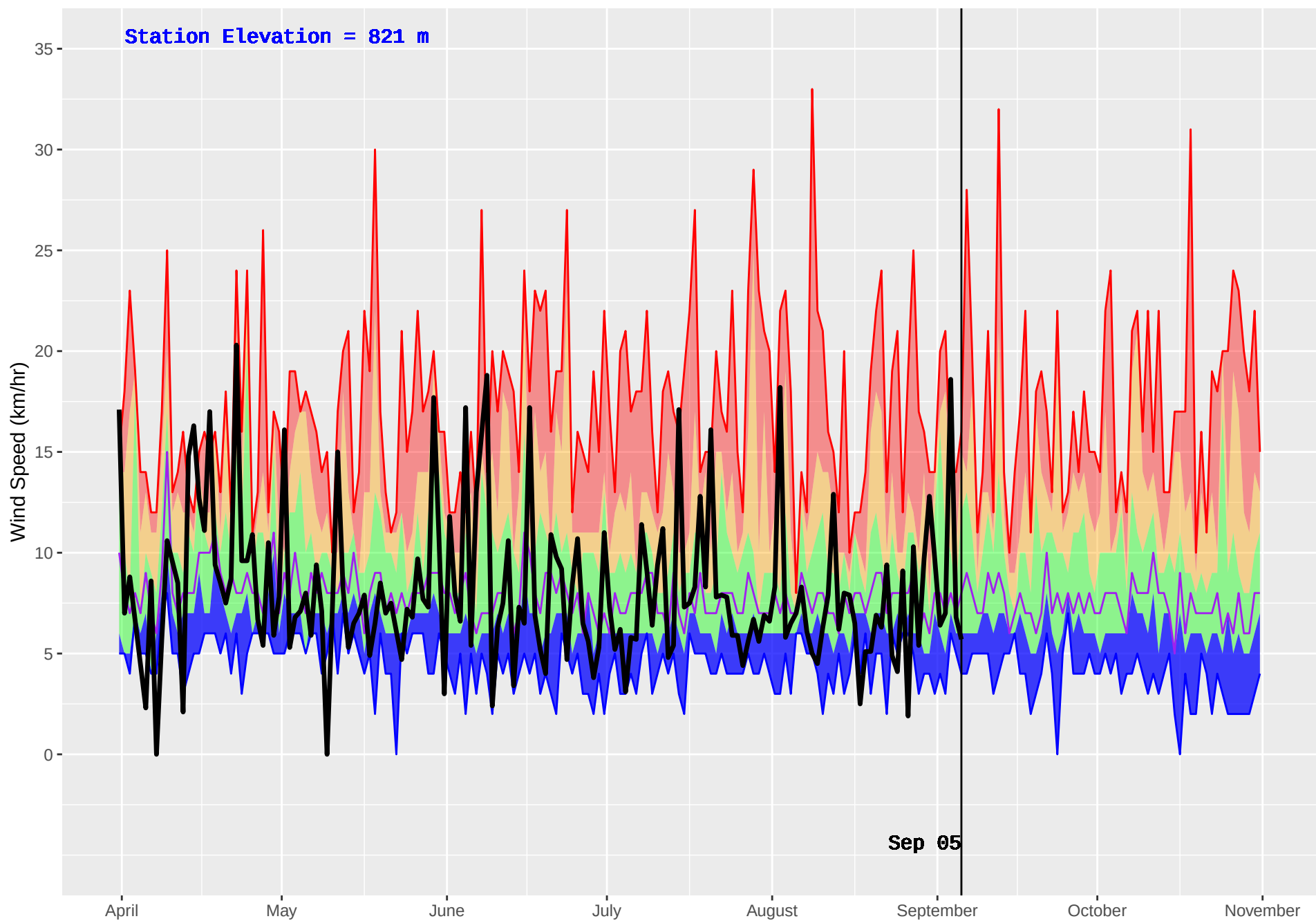
AKOKLI CREEK (838) : Historical (2003–2016) and Current (2018) Daily Wind Speed
